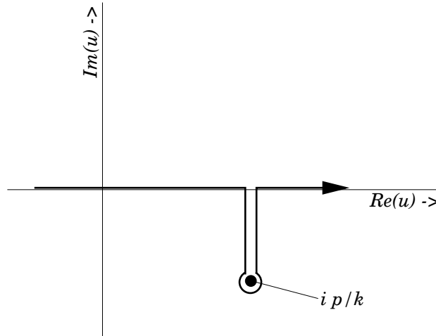
Figure 6.3: The Bromwich contour for Landau damping.
